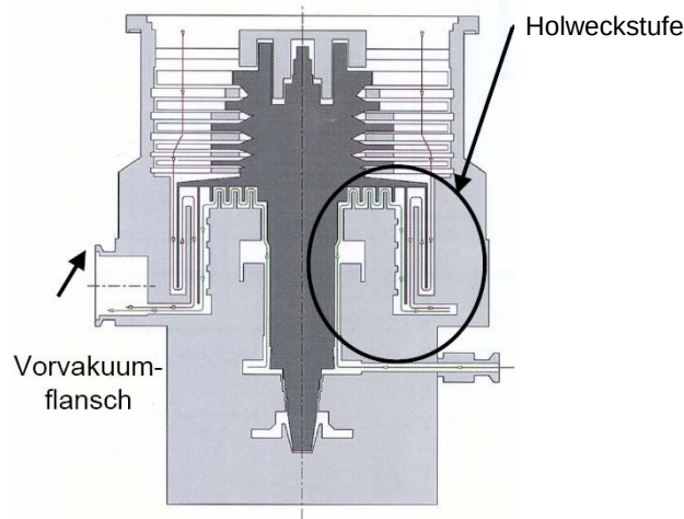
Figure A.10: Holweck stage of a turbomolecular pump.
