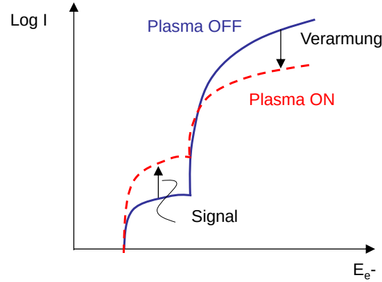
Figure 6.23: Signal curve in ionization threshold mass spectrometry.
