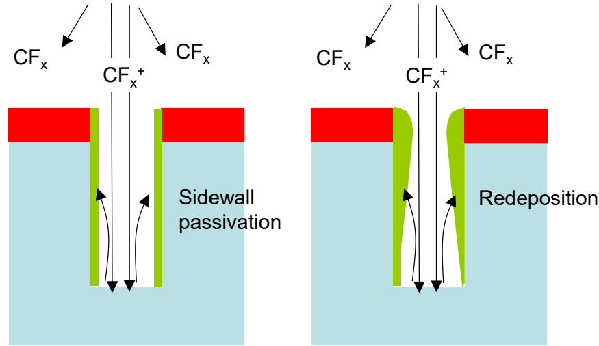
Figure 5.21: Sidewall passivation.
