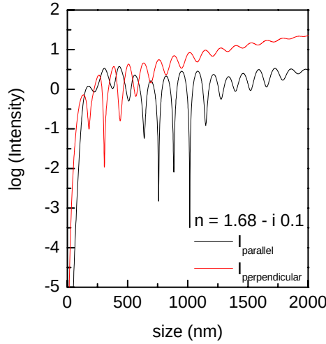
Figure C.2: Scattering intensities parallel and perpendicular to the plane of incidence for homogeneous spheres of varying size at a wavelength of 488 nm.
