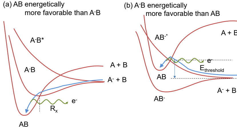
Figure 4.27: Associative detachment.
